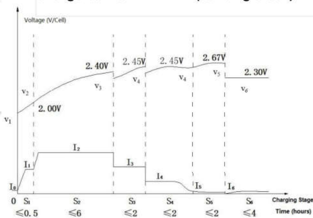
Charge Curve 12-DF-112 (for Single Cell)
