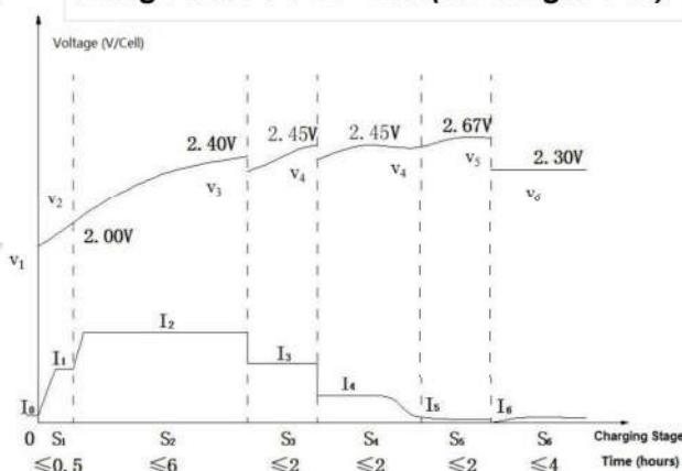
Charge Curve 6-DF-260 (for Single Cell)
